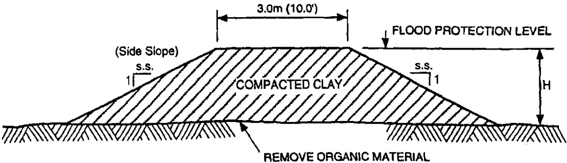
DIKE CROSS - SECTION (minimum elevations)
