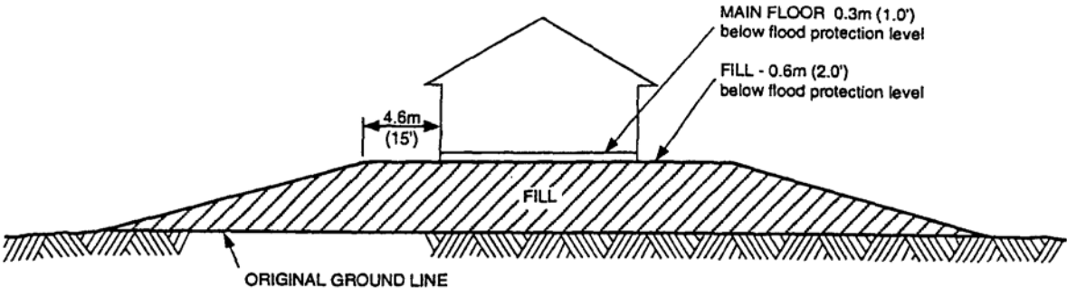
MACHINE SHED, WORK SHOP, GRANARY, STORAGE BUILDING (minimum elevations)
