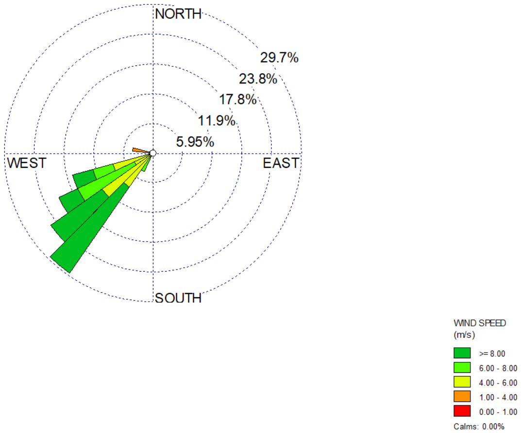
Figure B-3: Wind Rose – May 10, 2022
