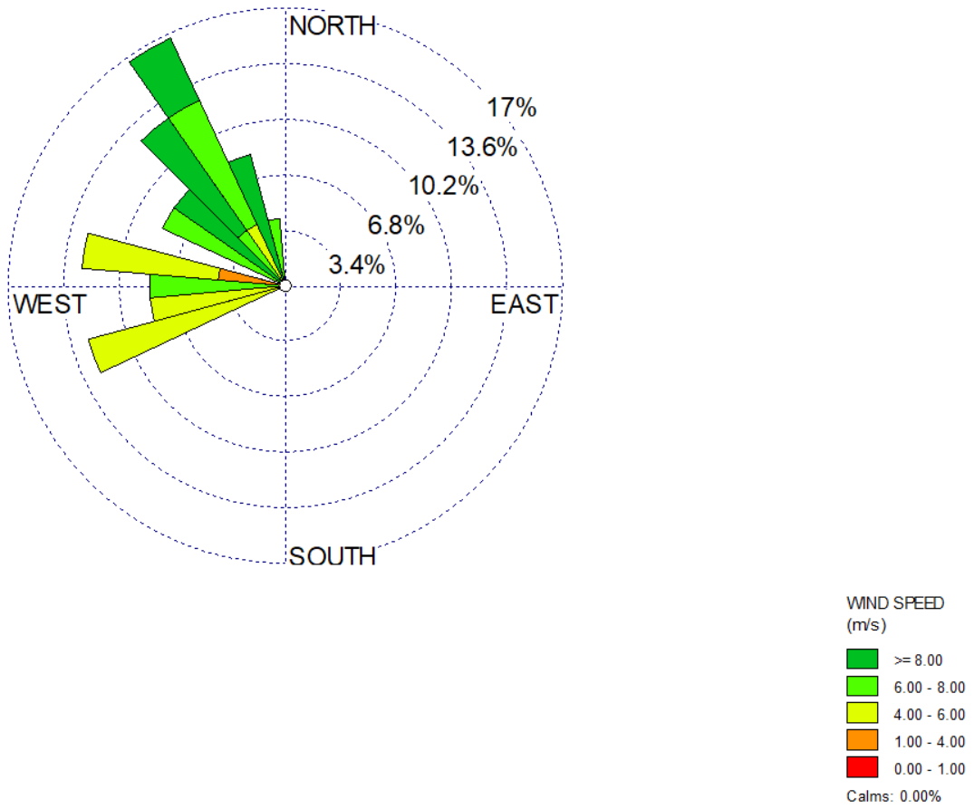
Figure B-7: Wind Rose – May 15, 2022
