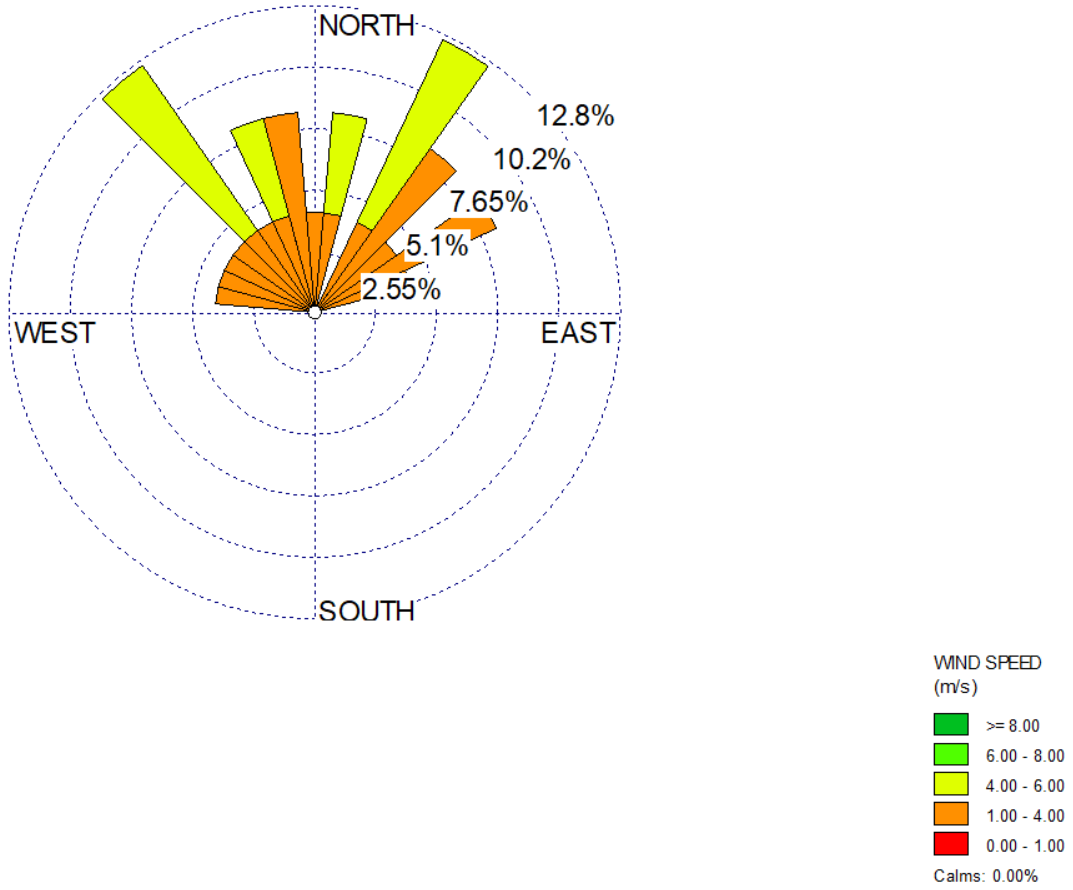
Figure B-8: Wind Rose – May 16, 2022
