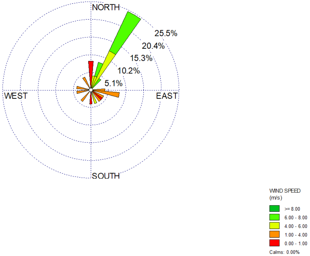
Figure B-4: Wind Rose – May 11, 2022
