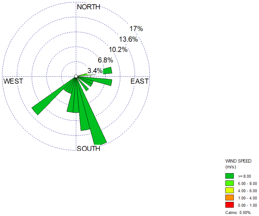
Figure B-5: Wind Rose – May 13, 2022
