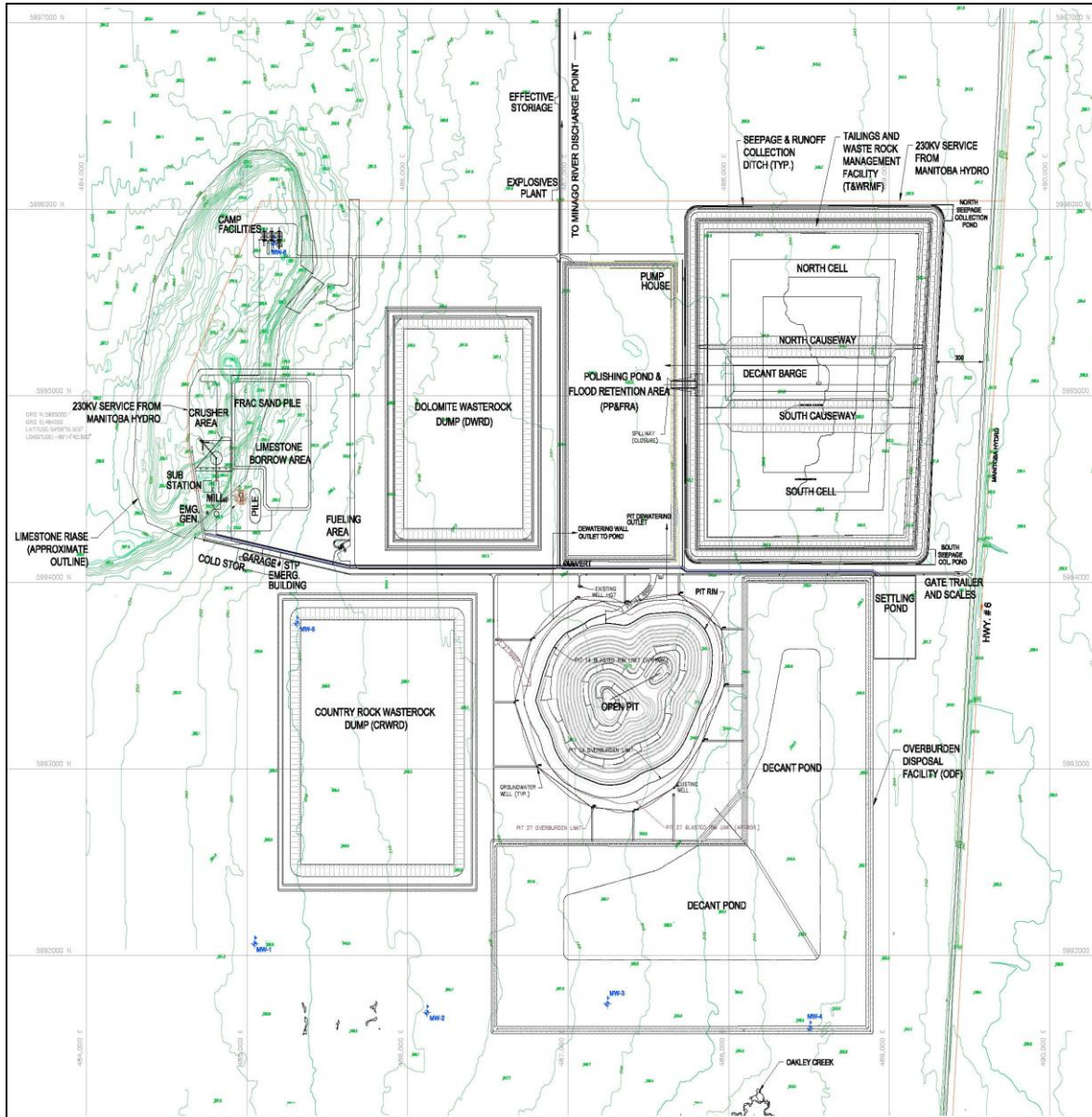
Figure 3.4-1 General Site Plan of Minago
