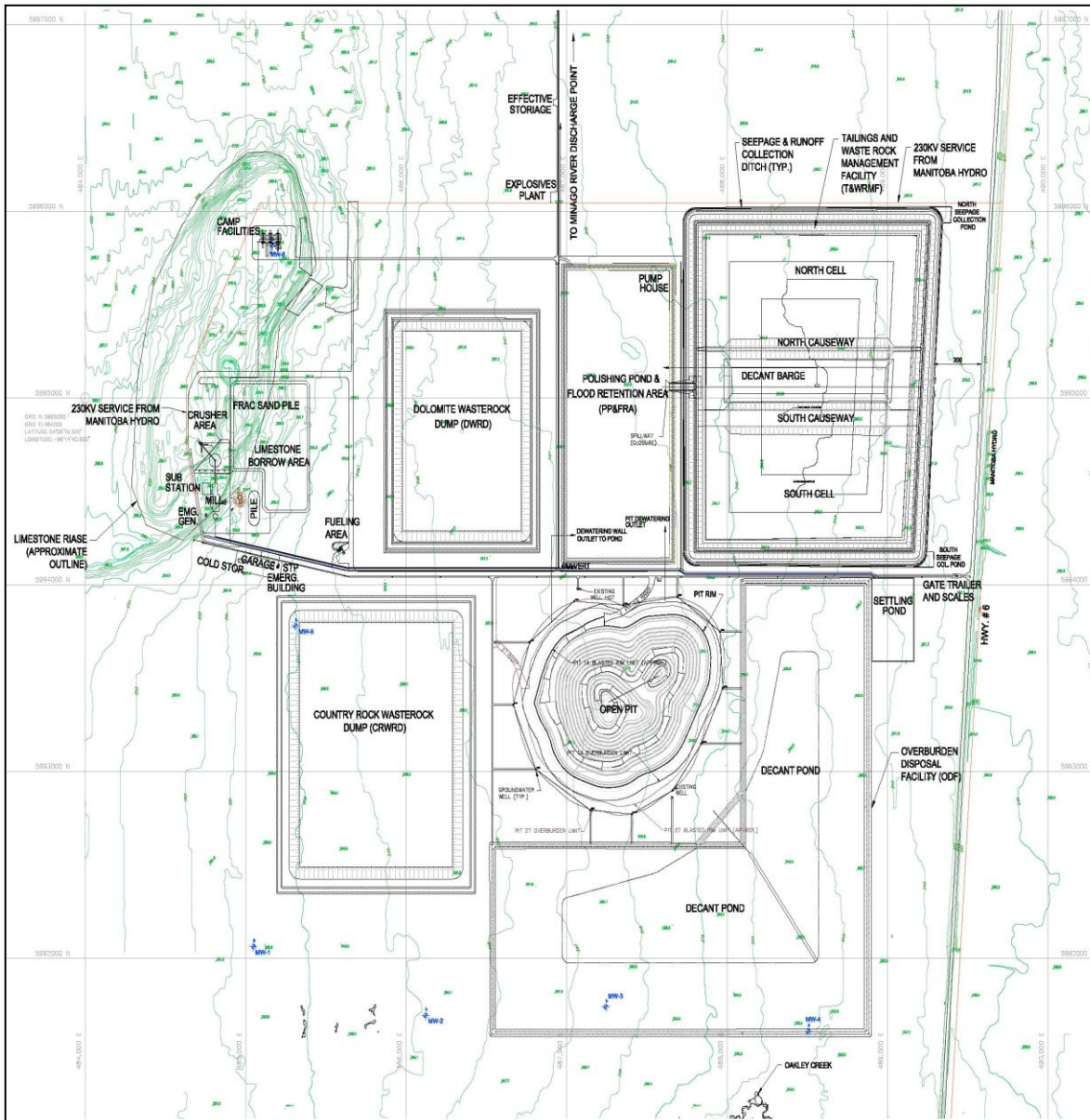
Figure 3.2-3 General Site Plan of Minago
