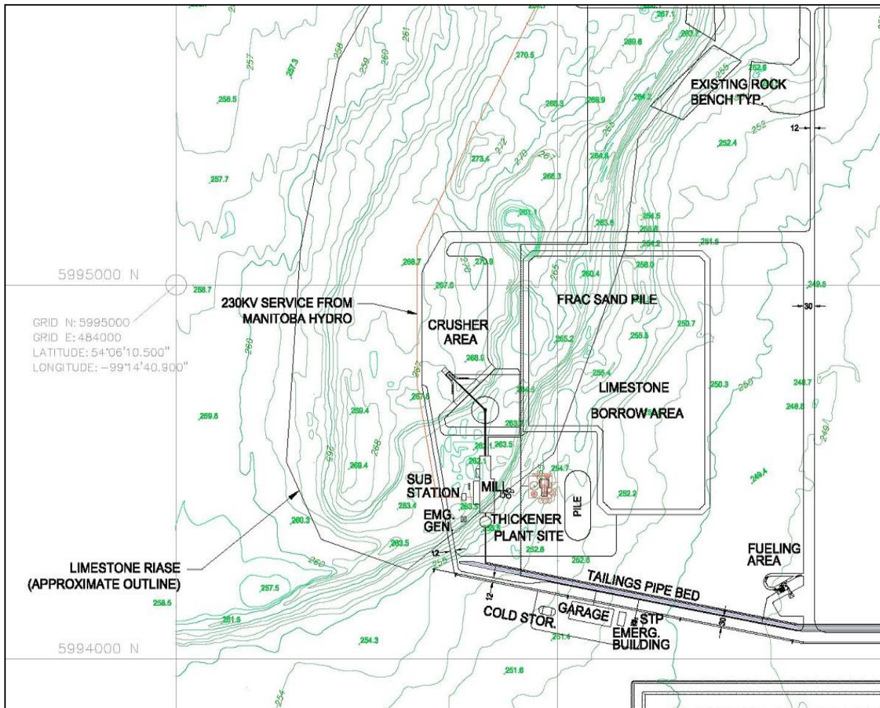
Figure 3.2-2 Minago Plant Area
