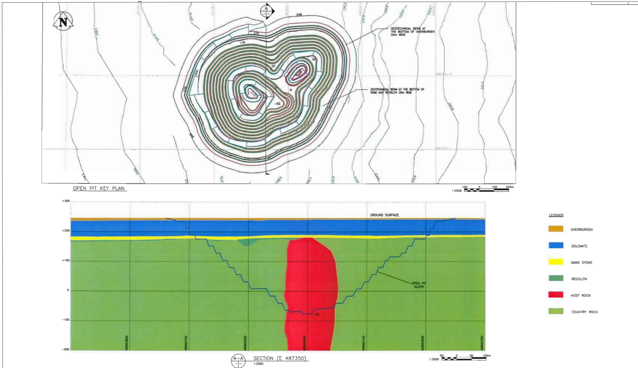
Figure 3.2-5 Ultimate Pit Design at Minago
