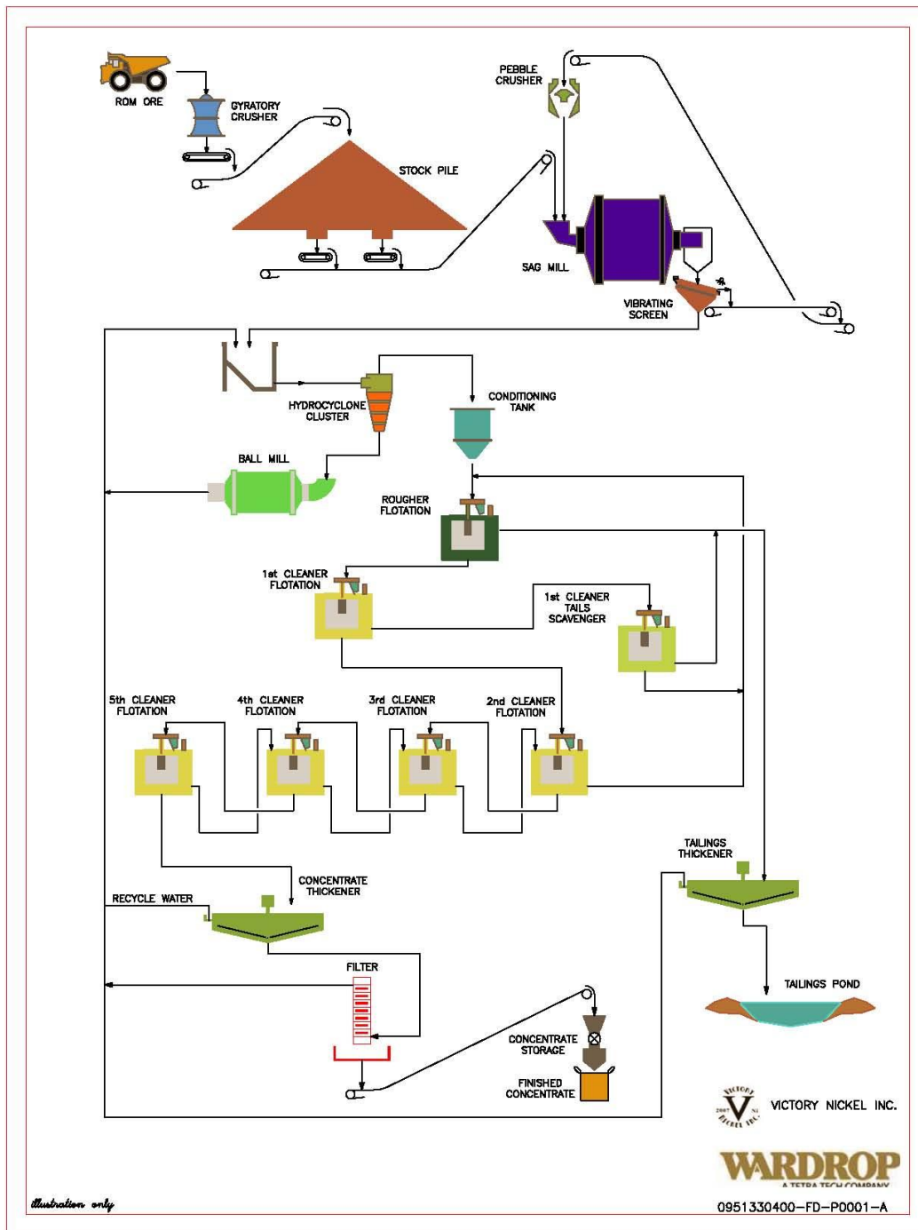
Figure 3.2-7 Simplified Flowsheet of the Nickel Ore Processing Plant
