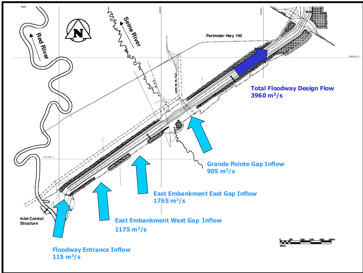
Figure 4.3-2 Flow Through Floodway Embankment Gaps for Design Flow
