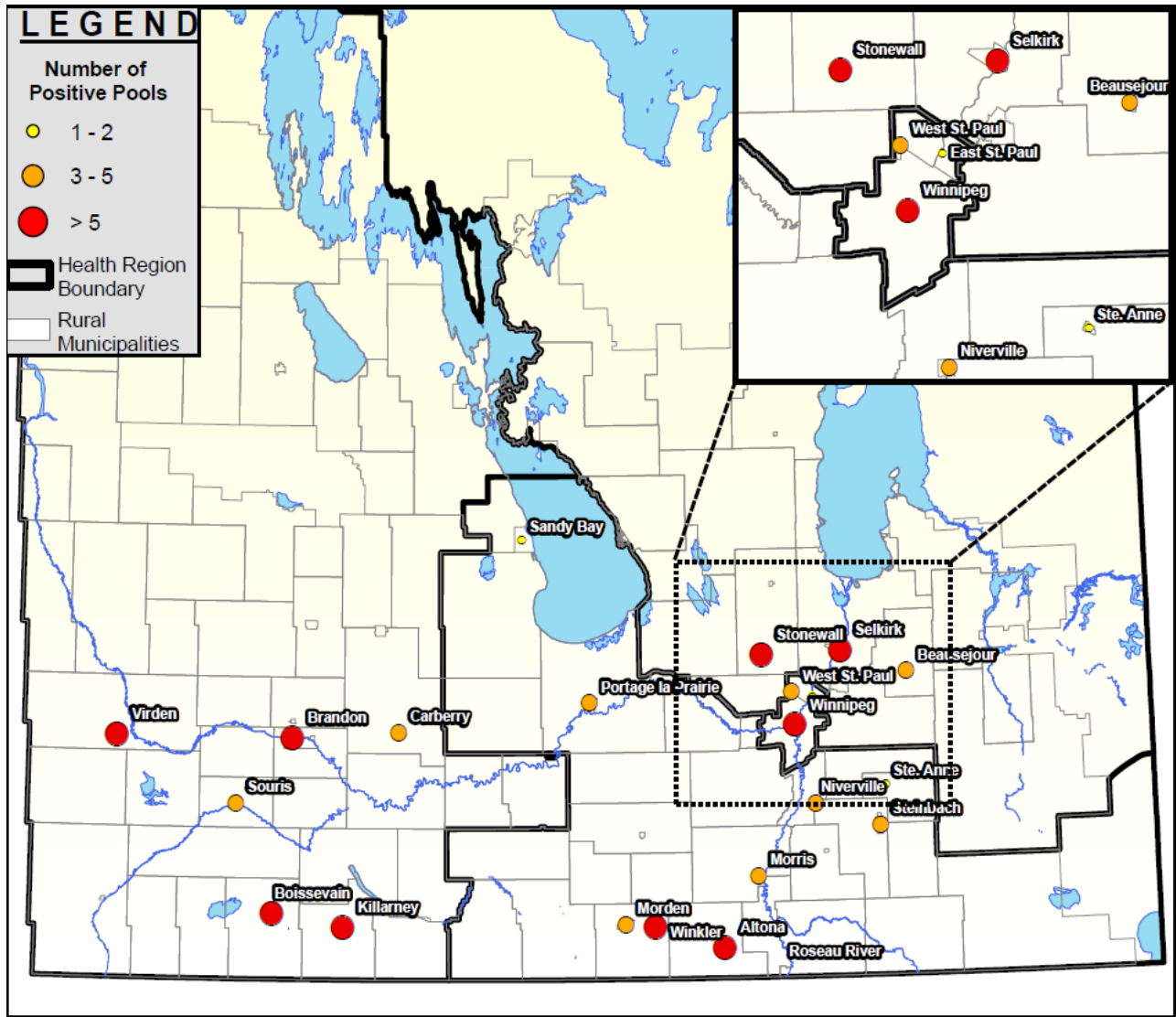
Figure 3 – Distribution of WNV positive Culex tarsalis mosquito pools collected in southern Manitoba (current to Week 34).
