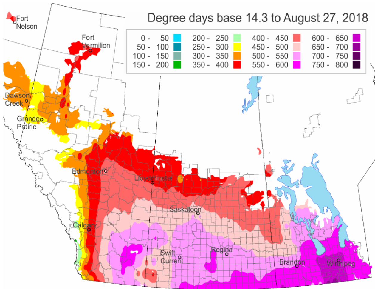
Figure 4 - Degree day accumulations, as of Week 34, across the Prairie Provinces
