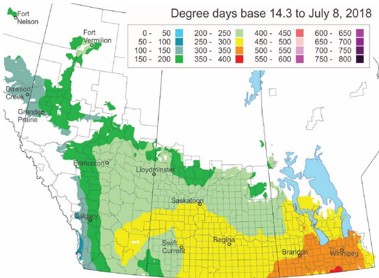
Figure 3 - Degree day accumulations, as of Week 27, across the Prairie Provinces.
