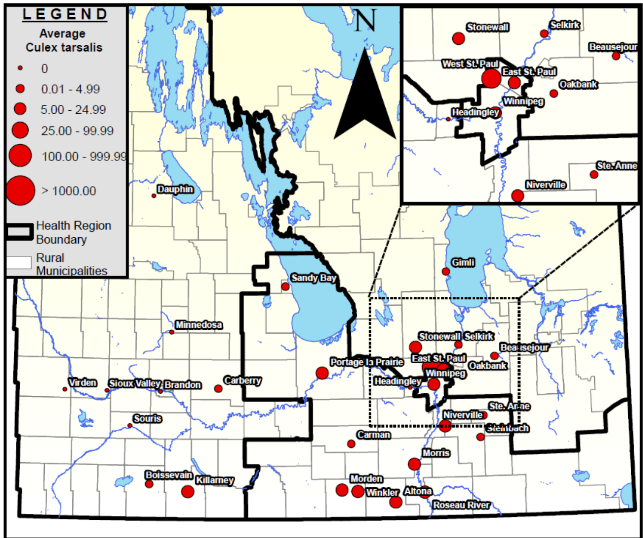
Figure 2 – Average number of Culex tarsalis mosquitoes collected across southern Manitoba during Week 23.
